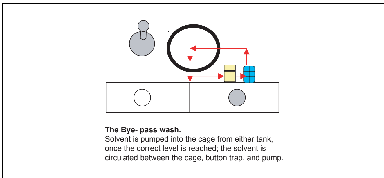
Figure 3.3: By pass wash for typical dry cleaning operation
